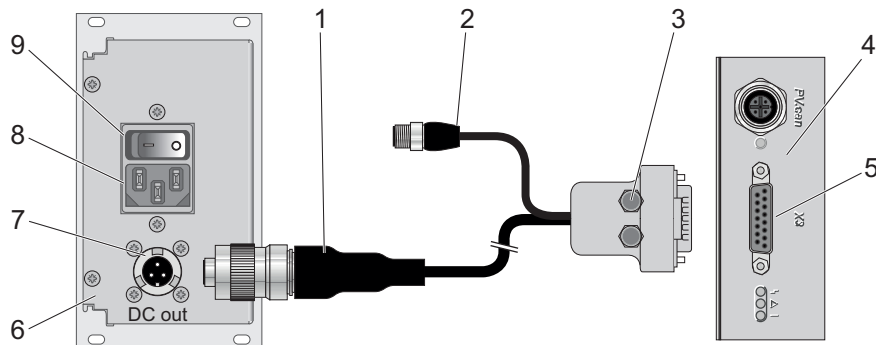
Fig. 14: Connecting electronic drive unit to power supply pack
