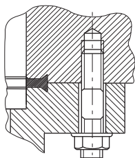
Fig. 9: Flange connection CF-F, stud screw and tapped hole
