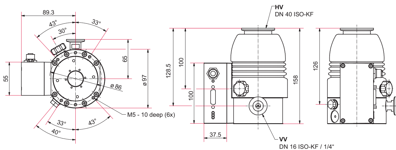
Fig. 21: Dimensions HiPace 80 | DN 40 ISO-KF
