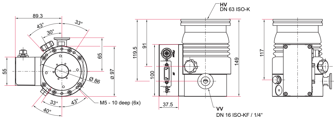
Fig. 19: Dimensions HiPace 80 | DN 63 ISO-K
