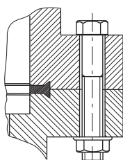
Fig. 8: Flange connection CF-F, hexagon head screw and through hole
