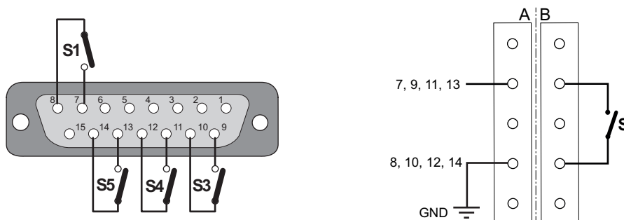
Fig. 5: Logic input wiring
