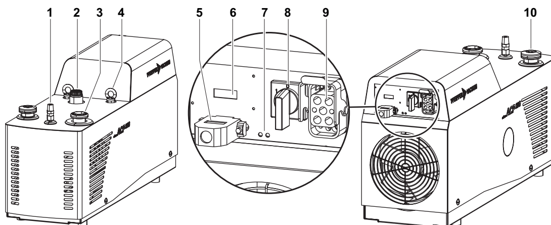
Fig. 4: ACP 28 - 40 with three-phase frequency converter
