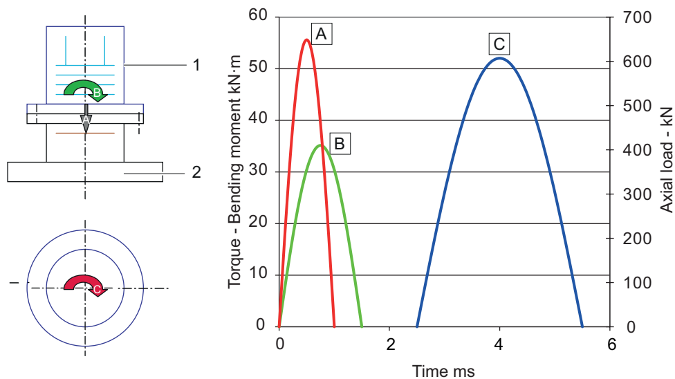
Fig. 4: Graph of the loads exerted on the equipment - ATH 2300 M
