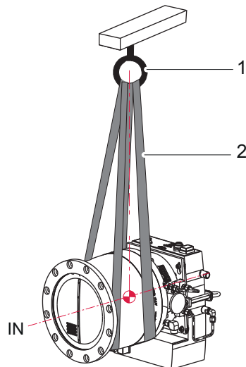
Fig. 5: Installing the pump horizontally
