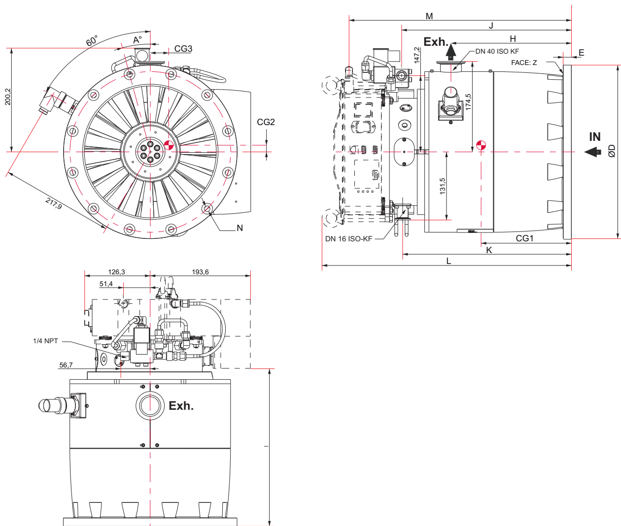
Fig. 10: Dimensions of ATH 2300 MT with OBC
