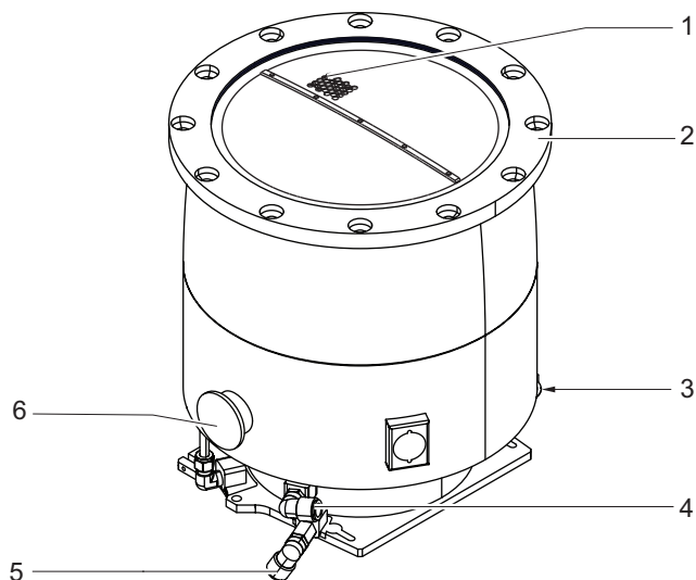
Fig. 1: Description of an ATH 2300 M pump
