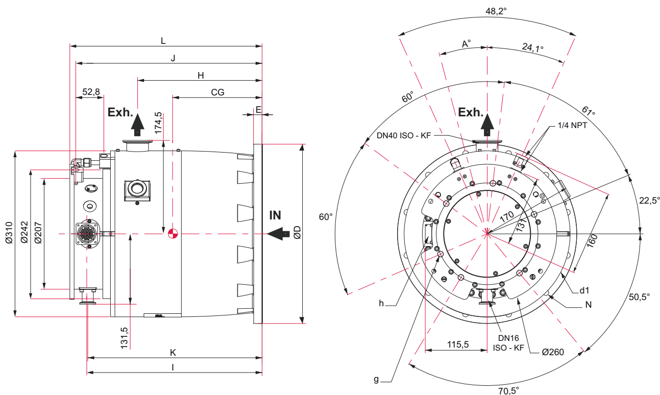
Fig. 8: ATH 2300 M dimensions
