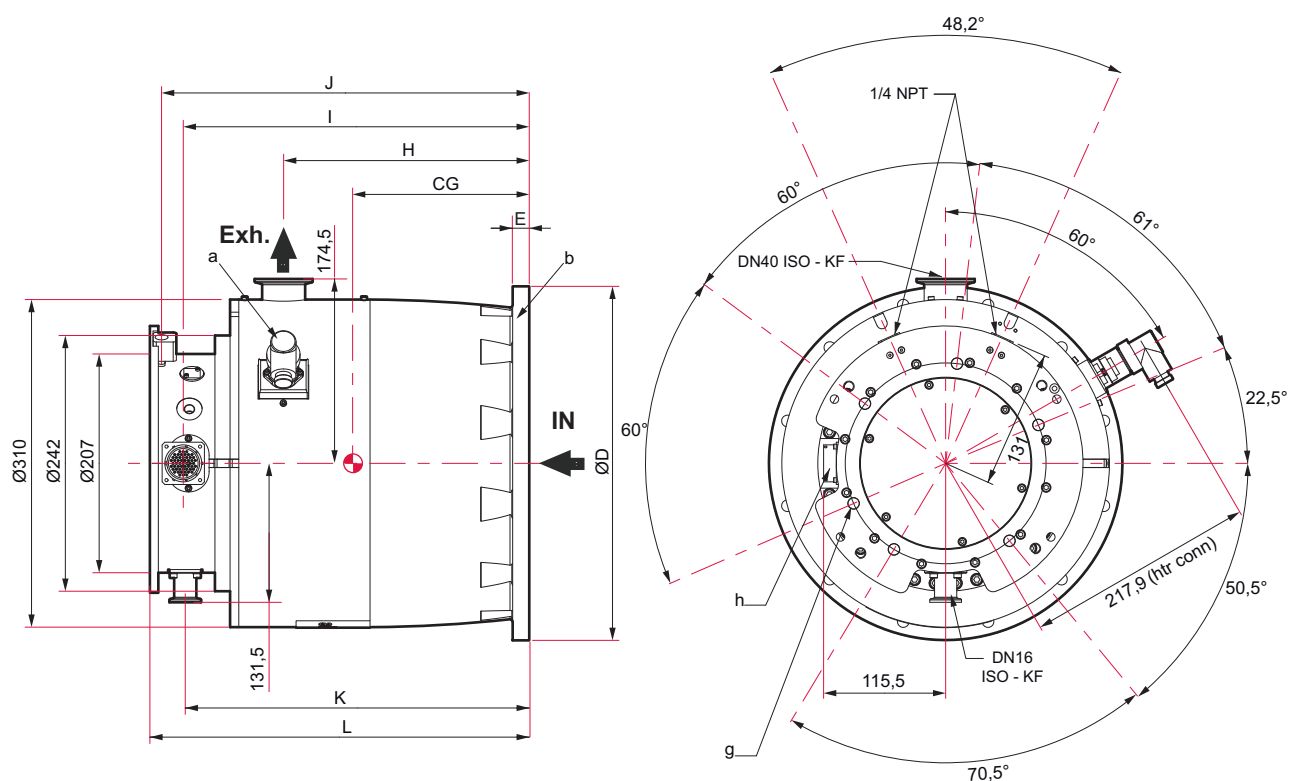
Fig. 9: ATH 2300 MT Dimensions
