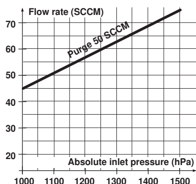
Fig. 7: Purge flow diagram
