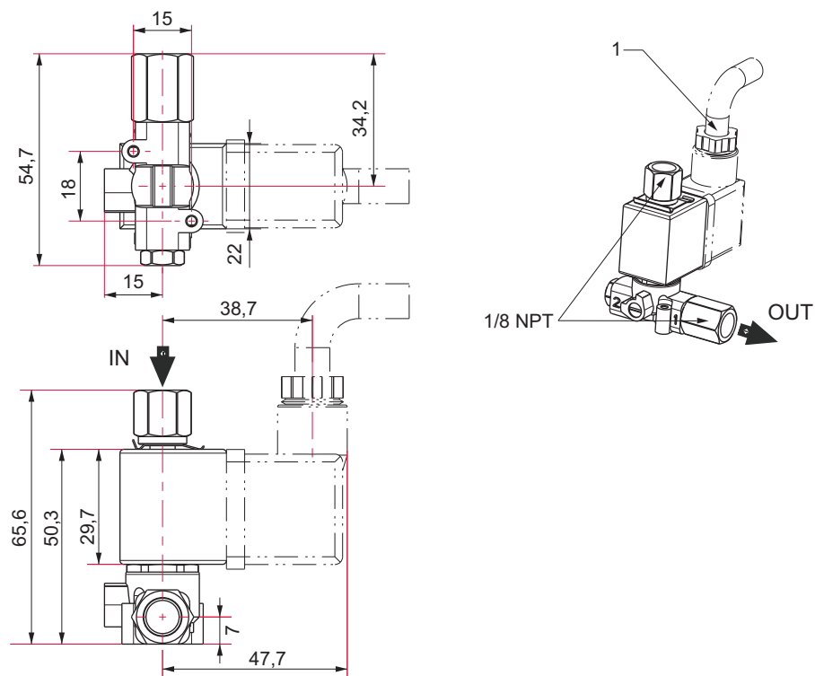
Fig. 13: Dimensions of water valve
