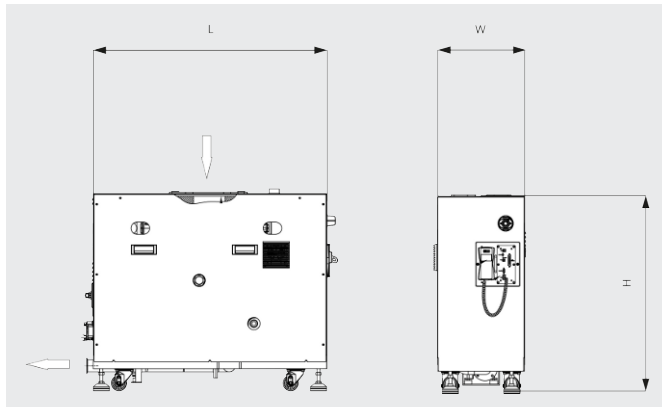
Dimensional drawing
