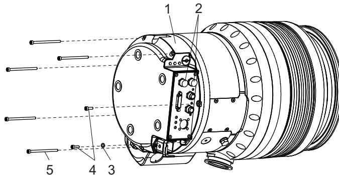
Fig. 28: Replacing the electronic drive unit – Fastening
