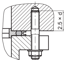
Fig. 13: Flange connection ISO-F, stud screw and tapped hole
