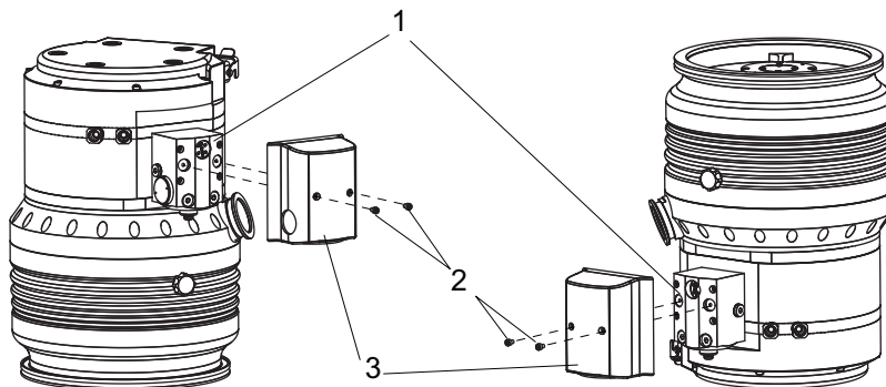
Fig. 23: Removing the protective cap on U- or standard versions
