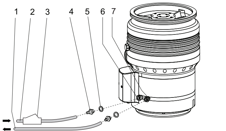
Fig. 21: Cooling water connection
