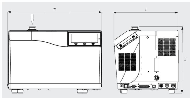
Dimensional drawing
